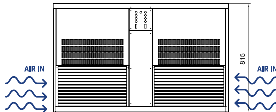
FRONTAL VIEW VISTA FRONTAL
